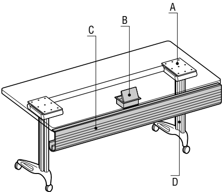
C Base • Flip Top A Flip Top Mechanism B Surface Power Unit C J Modesty/Wire Bin D Removable Base Cover Strip
