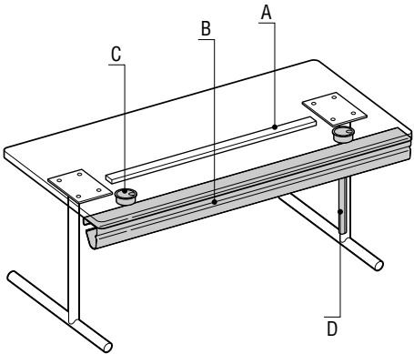
Tubular C Base • Fixed A Top Support Rail (when required) B Large Wire Manager C Grommet D Snap-on Leg Wire Manager
