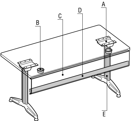
T Base • Folding Base A Folding Base Mechanism B Grommet C Flat Folding Modesty with: D Horizontal Wire Manager E Removable Base Cover Strip
