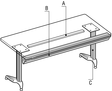
C Base • Fixed A Top Support Rail (when required) B Large Wire Manager C Removable Base Cover Strip
