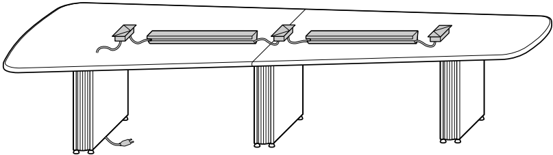
Three surface power units daisychained – single core drill. Horizontal cabling within Large Wire Managers.
