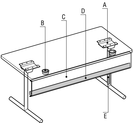
Tubular T Base • Folding Base A Folding Base Mechanism B Grommet C Flat Folding Modesty with: D Horizontal Wire Manager E Snap on Leg Wire Manager
