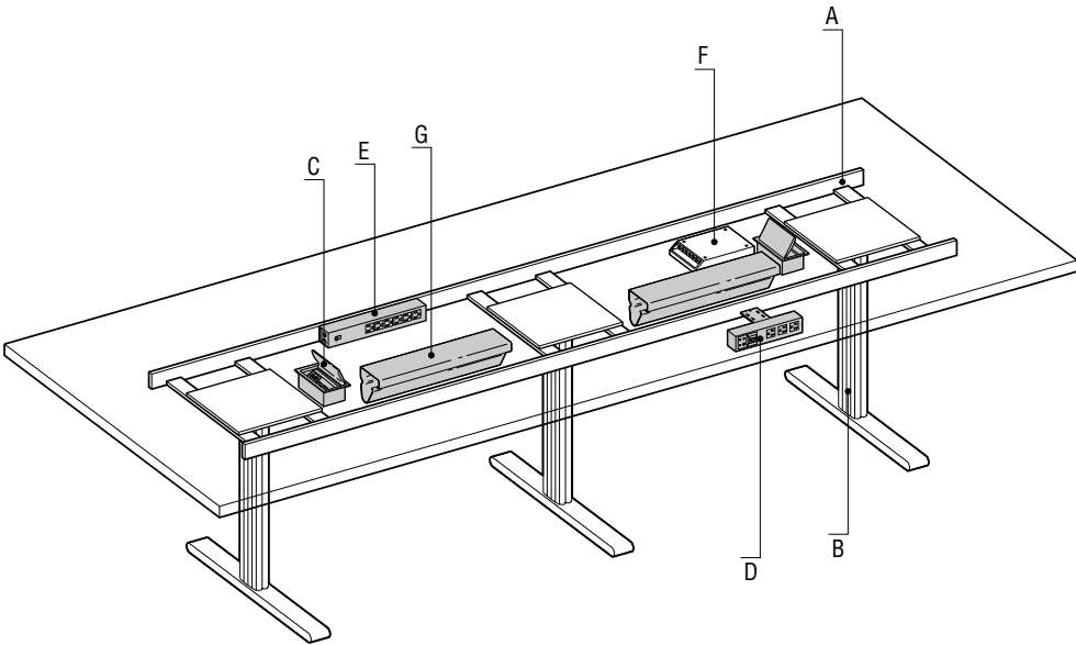
Kable T Base A Table Top Support Rail B Removable Wireway Strip C Surface Power Unit D Under top Power Unit E Surge Protected Power Bar F Data Hub (client supplied) G Large Wire Manager
