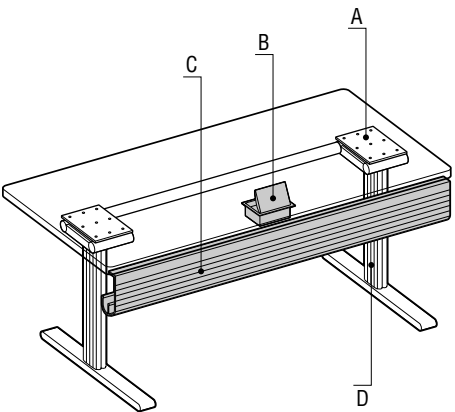
Kable T Base • Flip Top A Flip Top Mechanism B Surface Power Unit C J Modesty/Wire Bin D Removable Base Cover Strip
